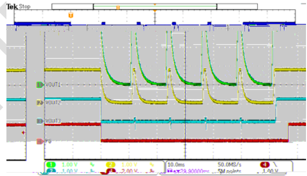
Figure 30. Buck3 Short-circuit and Recovery
