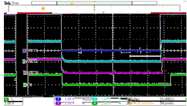
Figure 28. Buck1 Short-circuit and Recovery
