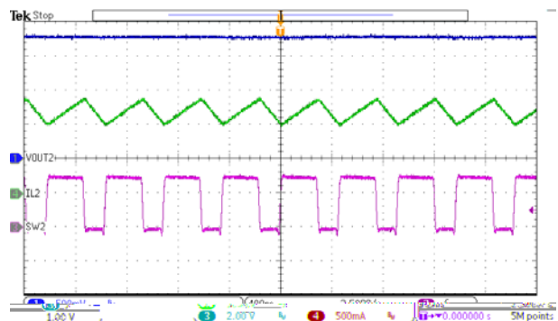
Figure 26. Buck2 Steady State, Load=1.2A
