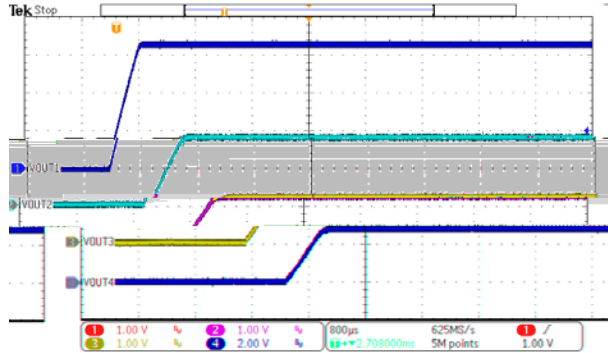
Figure 21. Power On Sequence I
