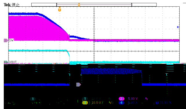
Figure 14. Power down(Iload=6A)
