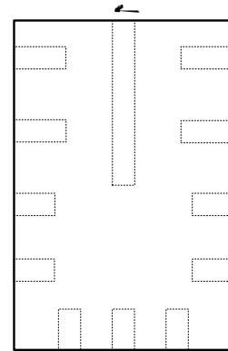
Figure 1. 12-Lead QFN 2mmx3mm
