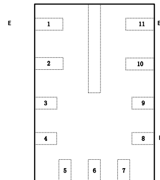
Figure 1. 12-Lead QFN 2mmx3mm
