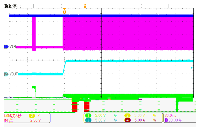
Figure 17. Over Current Release (hard short to 1A )
