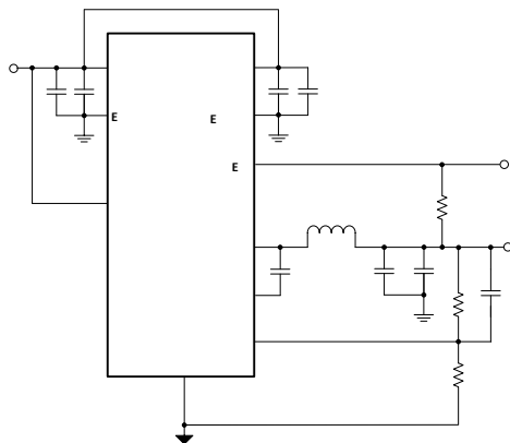
3.6V-36V, Synchronous Buck Converter
