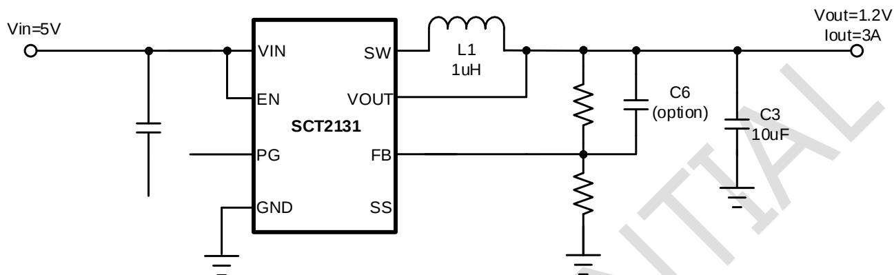
Figure 8. SCT2131 Design Example, 1.2V Output
