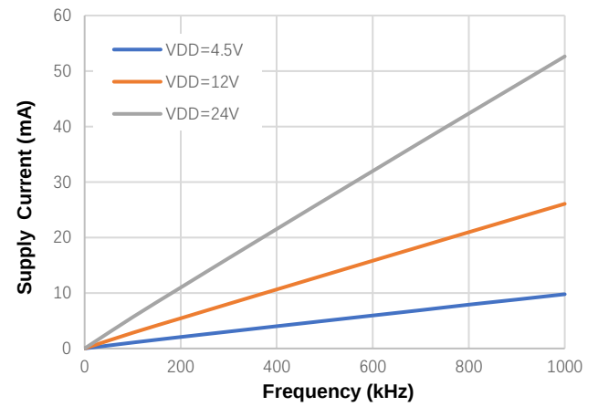
Figure 10. Operation Supply Current vs Frequency, C OUT =1nF
