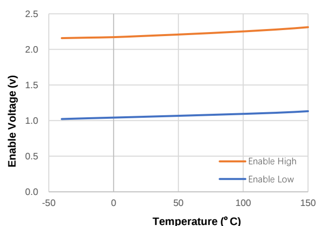
Figure 4. INA- and INB- Threshold vs Temperature
