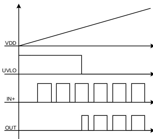
Figure 11. SCT52246 Output Vs VDD
