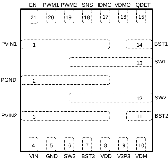
Figure 1. Top view 21-Lead QFN 4mm*4mm
