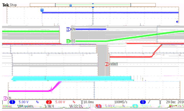
Figure 8. Power Up
