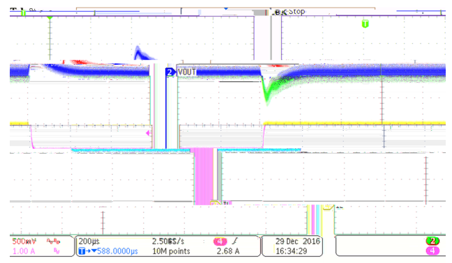
Figure 9. Load Transient ( I_{out}=2A to 3A , SR=250mA/\mu s )
