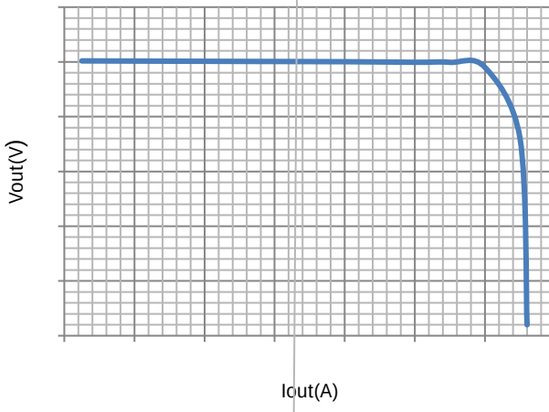
Figure 5. 5V LDO Iout vs Vout
